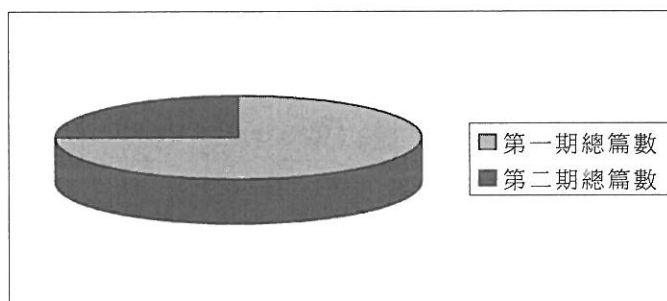
Fig 1 Statistics
