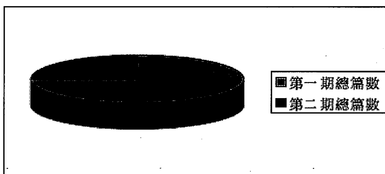
Fig 1 Statistics
